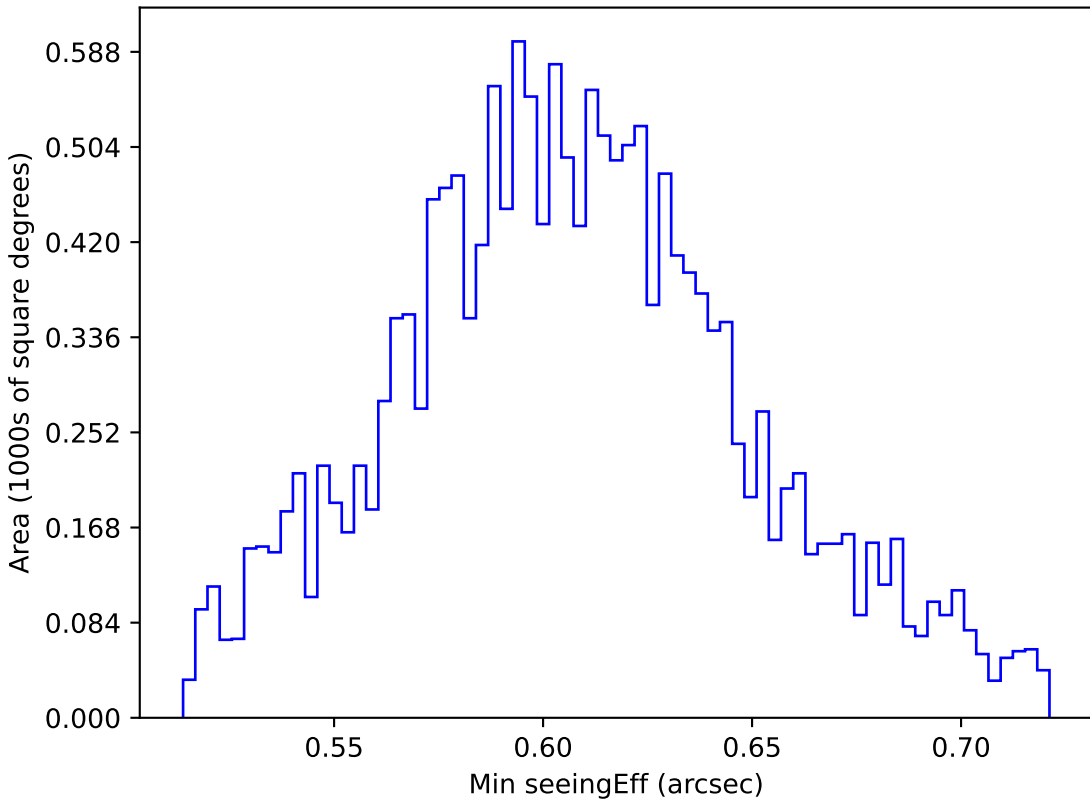
too_elab_r16_d2_giz_v3.4_10yrs WFD i band: Min seeingEff
