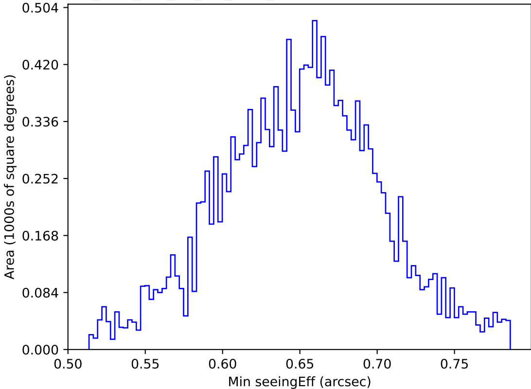
too_elab_r16_d2_giz_v3.4_10yrs WFD g band: Min seeingEff
