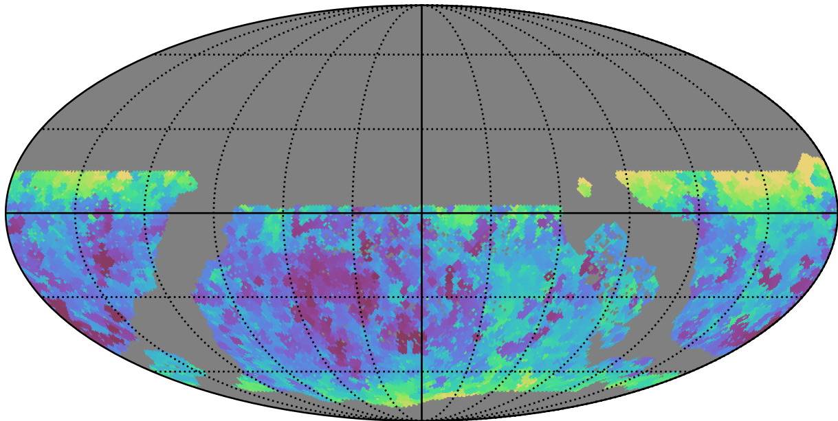
too_elab_r16_d2_giz_v3.4_10yrs WFD all bands: Min seeingEff
