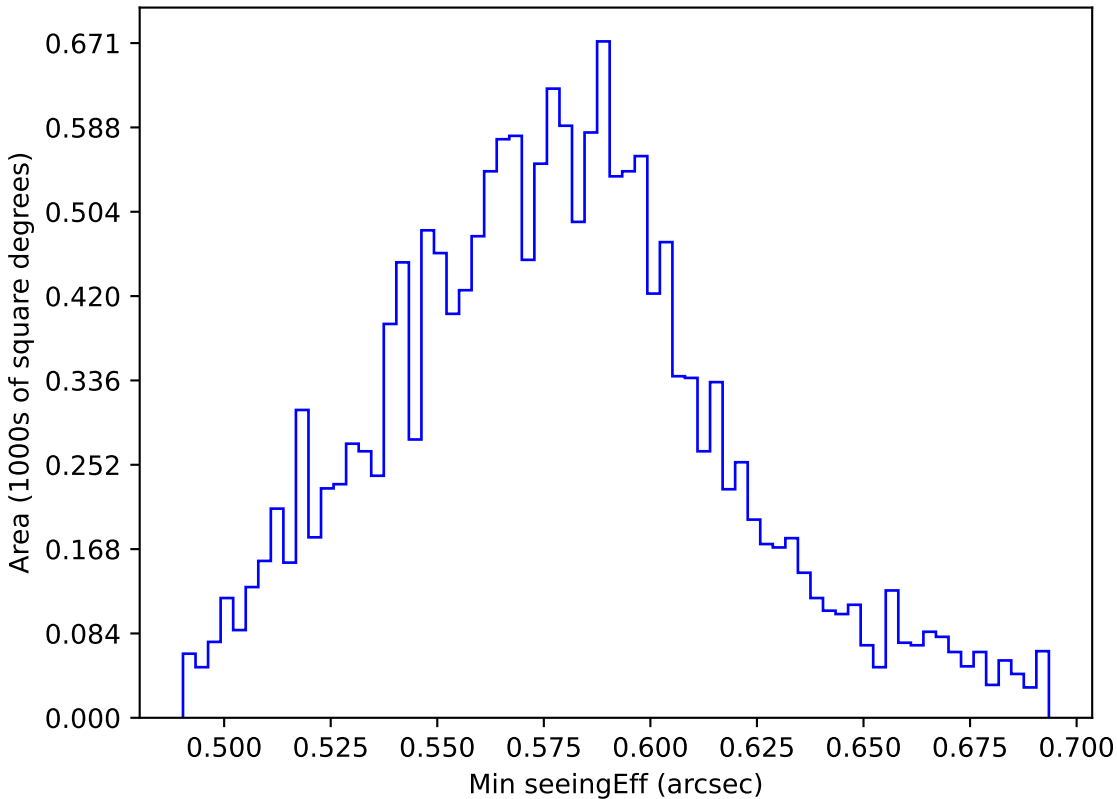
too_elab_r16_d2_giz_v3.4_10yrs WFD all bands: Min seeingEff
