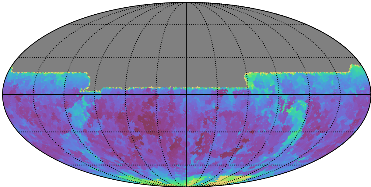
too_elab_r16_d2_giz_v3.4_10yrs All sky y band: Min seeingEff
