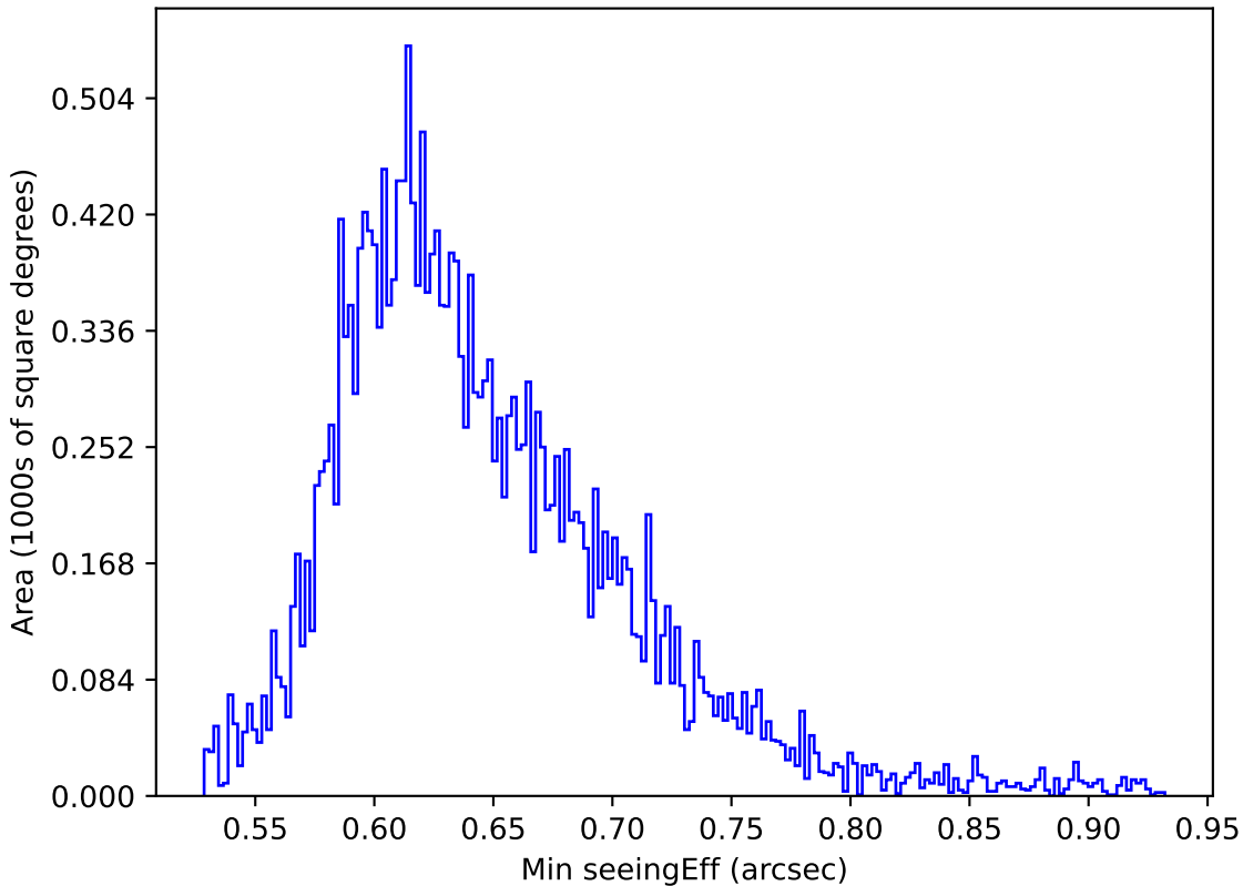
too_elab_r16_d2_giz_v3.4_10yrs All sky y band: Min seeingEff
