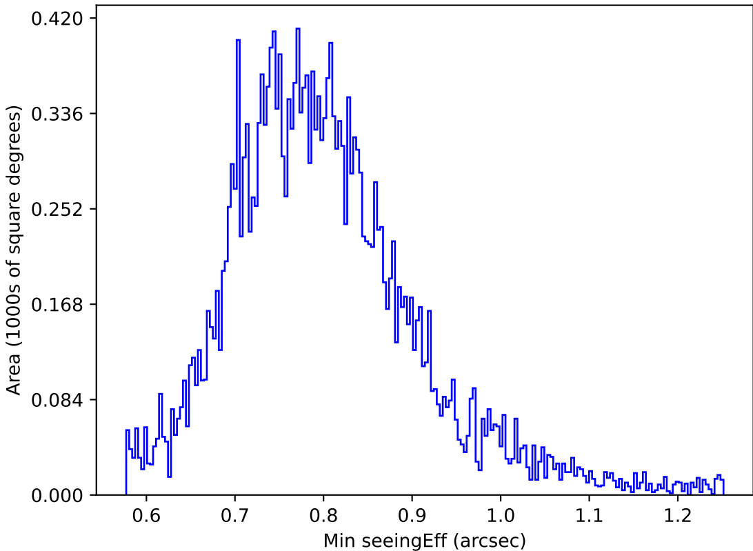
too_elab_r16_d2_giz_v3.4_10yrs All sky u band: Min seeingEff
