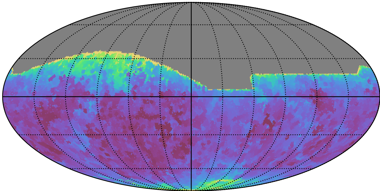
too_elab_r16_d2_giz_v3.4_10yrs All sky i band: Min seeingEff
