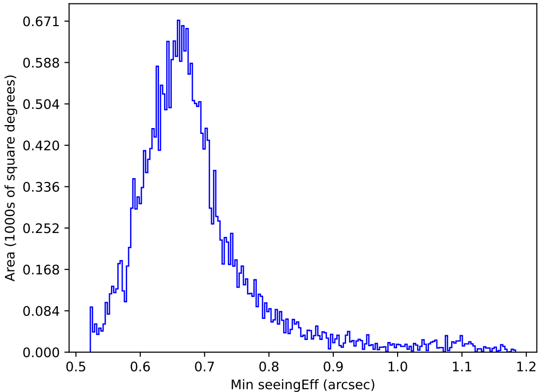
too_elab_r16_d2_giz_v3.4_10yrs All sky g band: Min seeingEff
