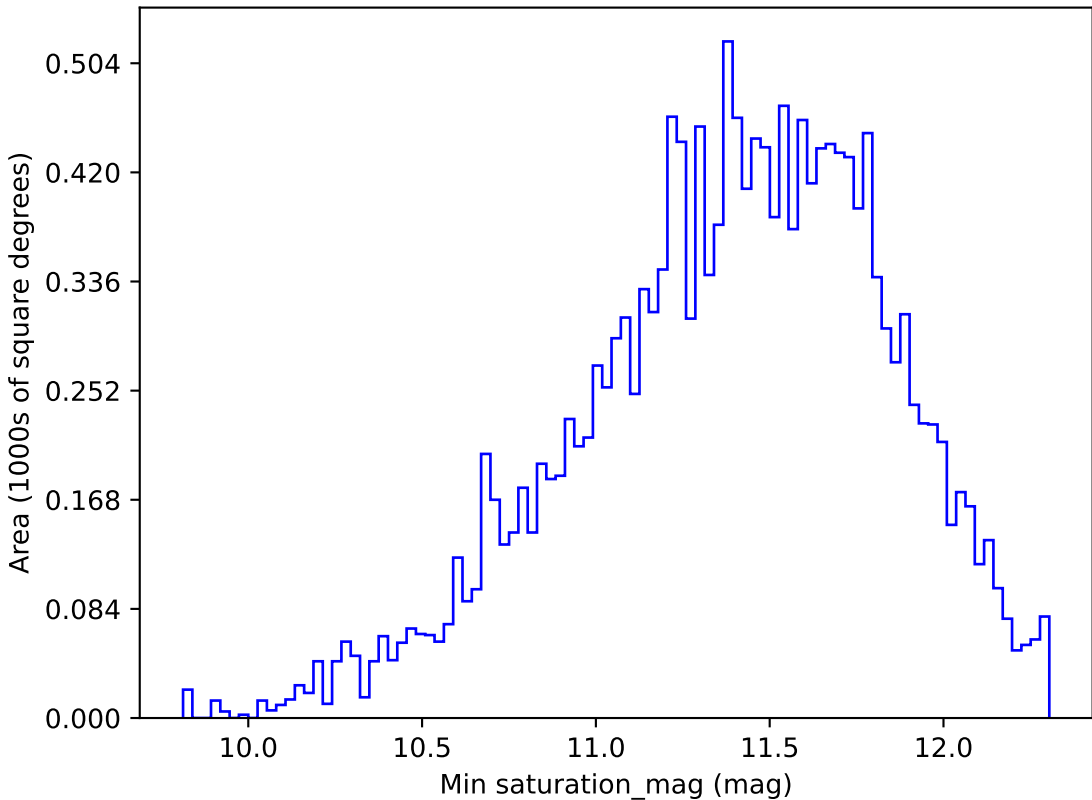
too_elab_r16_d2_giz_v3.4_10yrs WFD u band: Min saturation_mag
