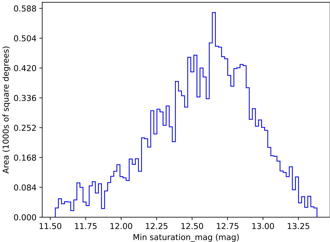
too_elab_r16_d2_giz_v3.4_10yrs WFD r band: Min saturation_mag
