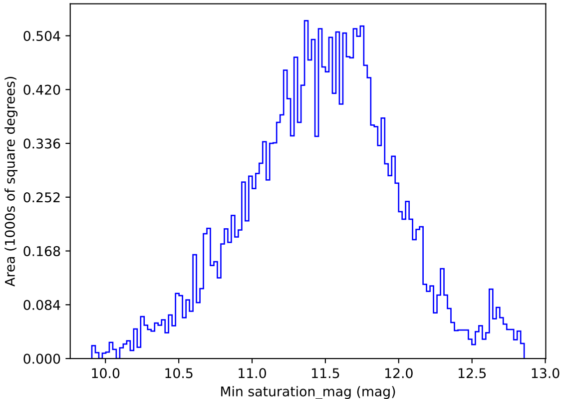
too_elab_r16_d2_giz_v3.4_10yrs All sky u band: Min saturation_mag
