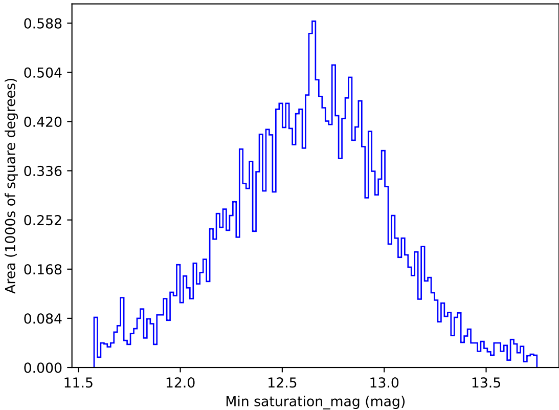
too_elab_r16_d2_giz_v3.4_10yrs All sky r band: Min saturation_mag
