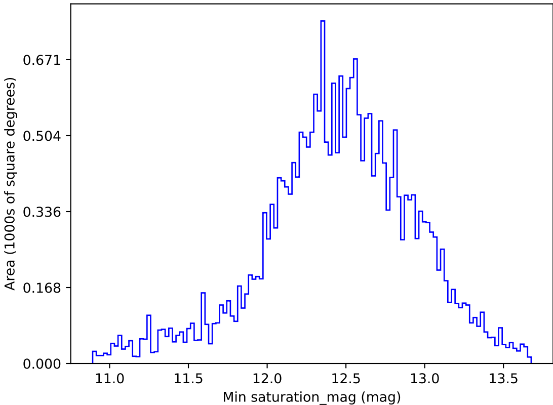
too_elab_r16_d2_giz_v3.4_10yrs All sky i band: Min saturation_mag
