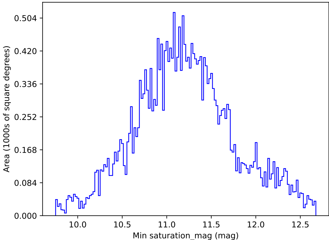
too_elab_r16_d2_giz_v3.4_10yrs All sky all bands: Min saturation_mag
