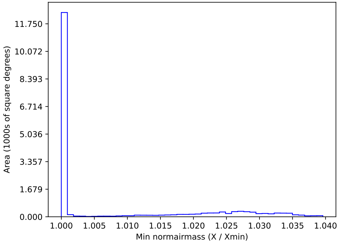
too_elab_r16_d2_giz_v3.4_10yrs WFD y band: Min normairmass
