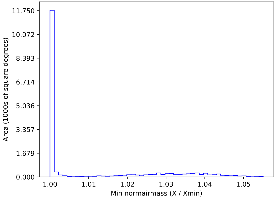
too_elab_r16_d2_giz_v3.4_10yrs WFD u band: Min normairmass
