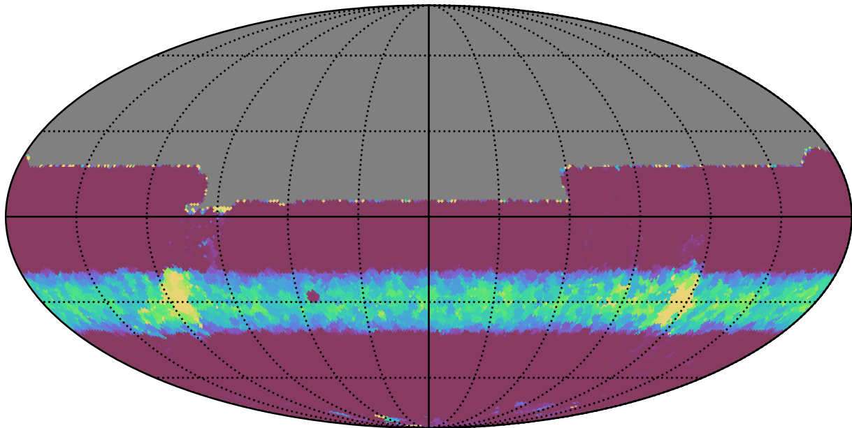
too_elab_r16_d2_giz_v3.4_10yrs All sky y band: Min normairmass
