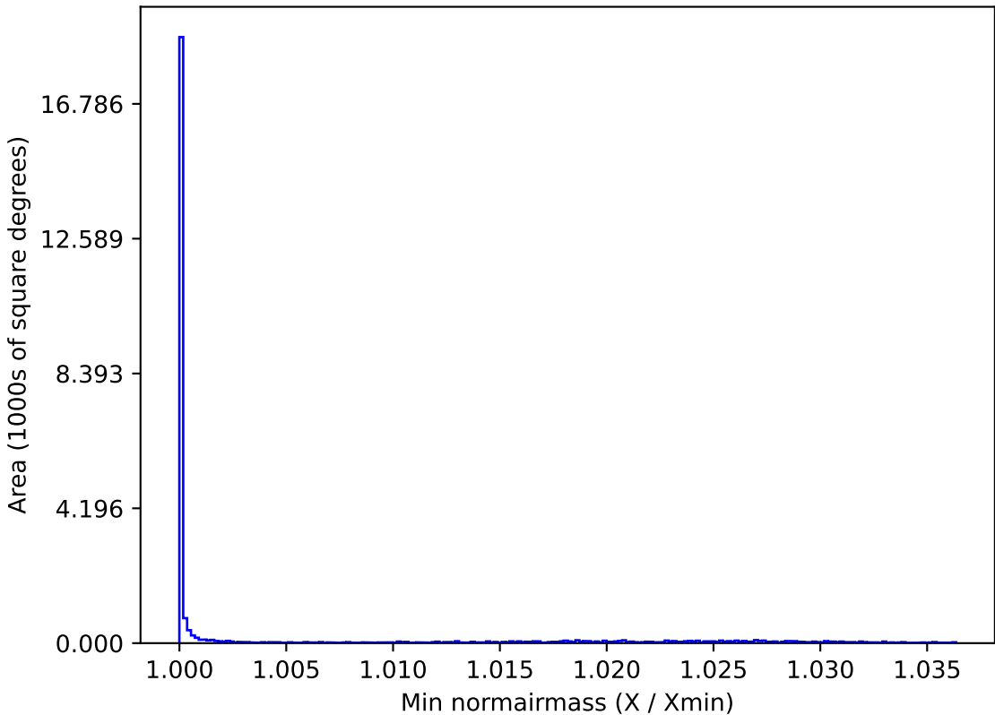
too_elab_r16_d2_giz_v3.4_10yrs All sky r band: Min normairmass
