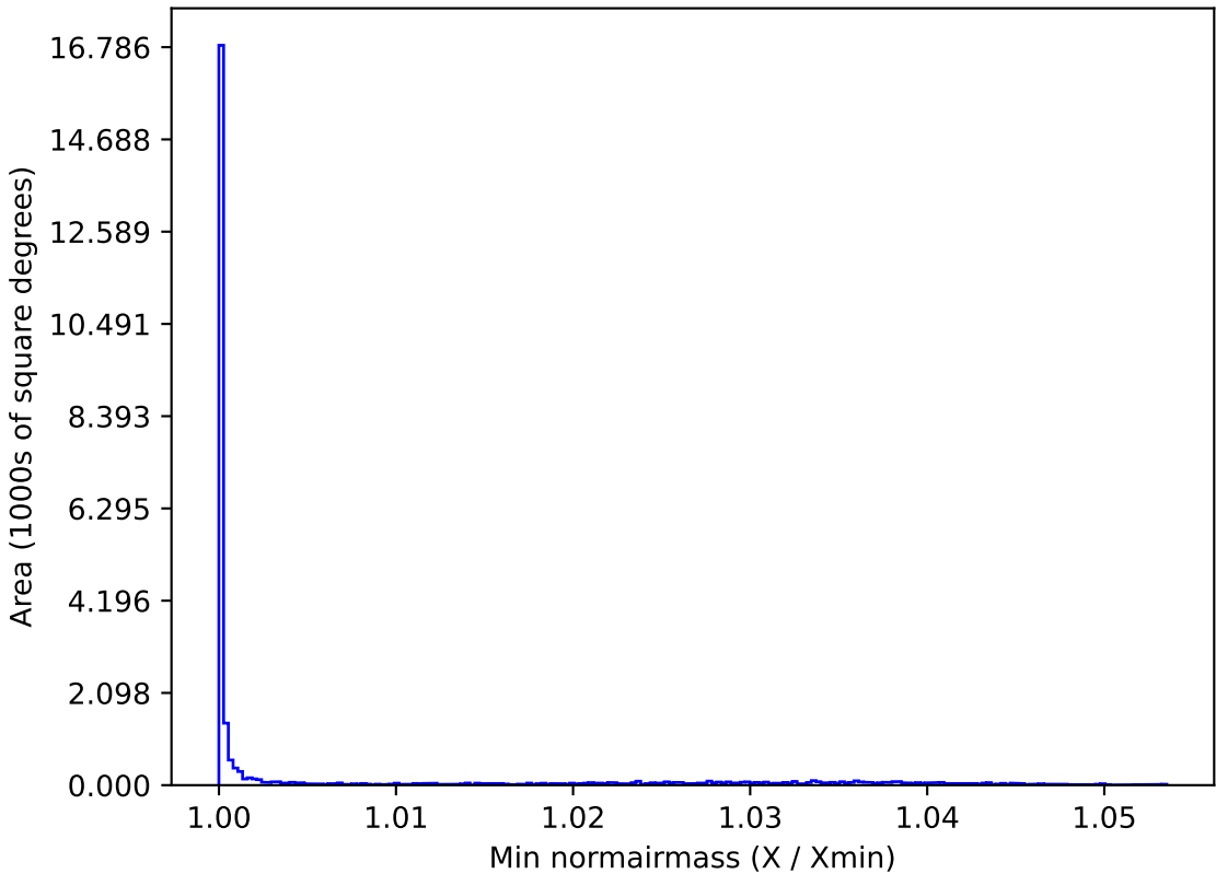
too_elab_r16_d2_giz_v3.4_10yrs All sky g band: Min normairmass
