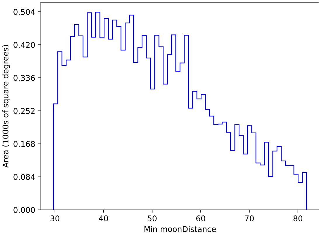
too_elab_r16_d2_giz_v3.4_10yrs WFD u band: Min moonDistance
