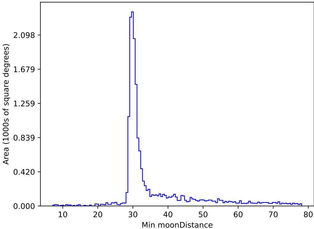
too_elab_r16_d2_giz_v3.4_10yrs WFD i band: Min moonDistance
