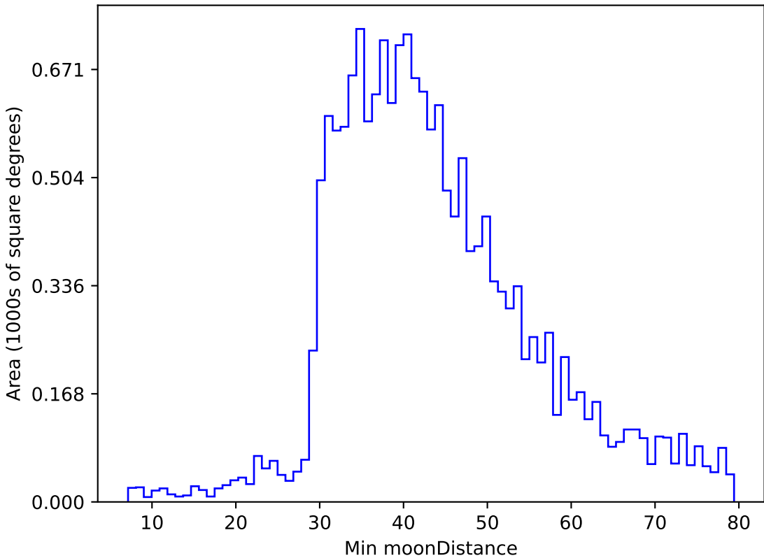
too_elab_r16_d2_giz_v3.4_10yrs WFD g band: Min moonDistance
