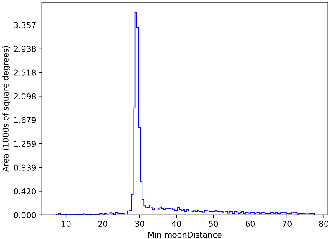
too_elab_r16_d2_giz_v3.4_10yrs WFD all bands: Min moonDistance
