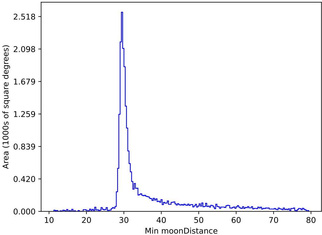
too_elab_r16_d2_giz_v3.4_10yrs All sky z band: Min moonDistance
