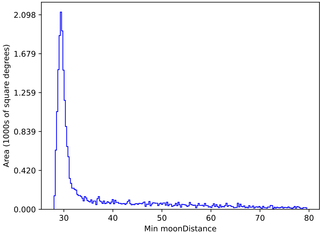
too_elab_r16_d2_giz_v3.4_10yrs All sky y band: Min moonDistance
