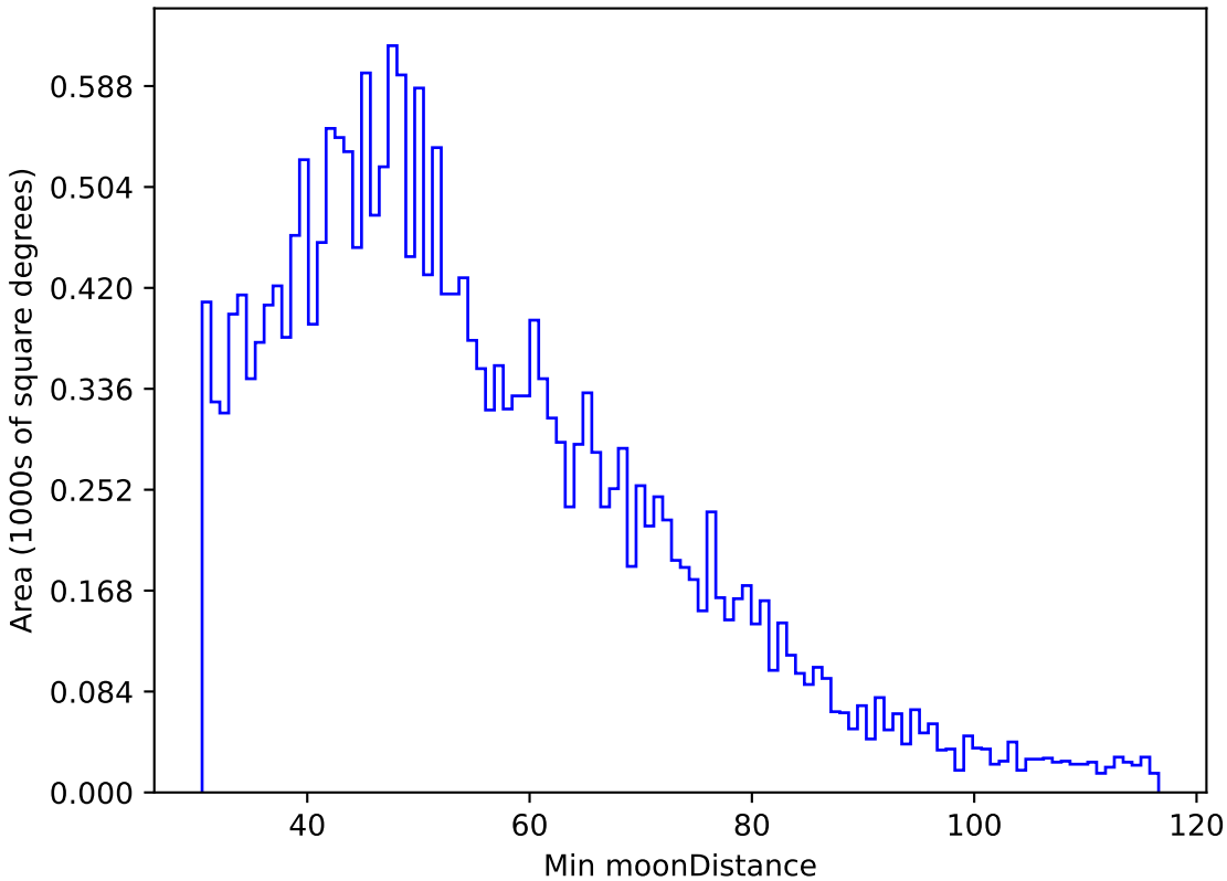
too_elab_r16_d2_giz_v3.4_10yrs All sky u band: Min moonDistance
