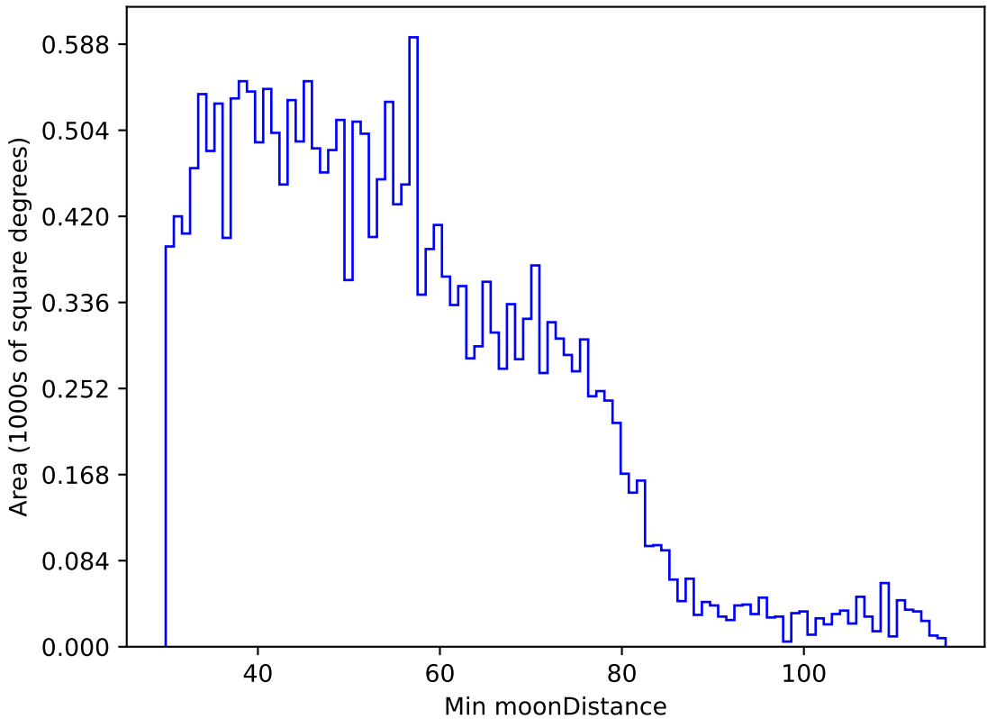
too_elab_r16_d2_giz_v3.4_10yrs All sky u band: Min moonDistance
