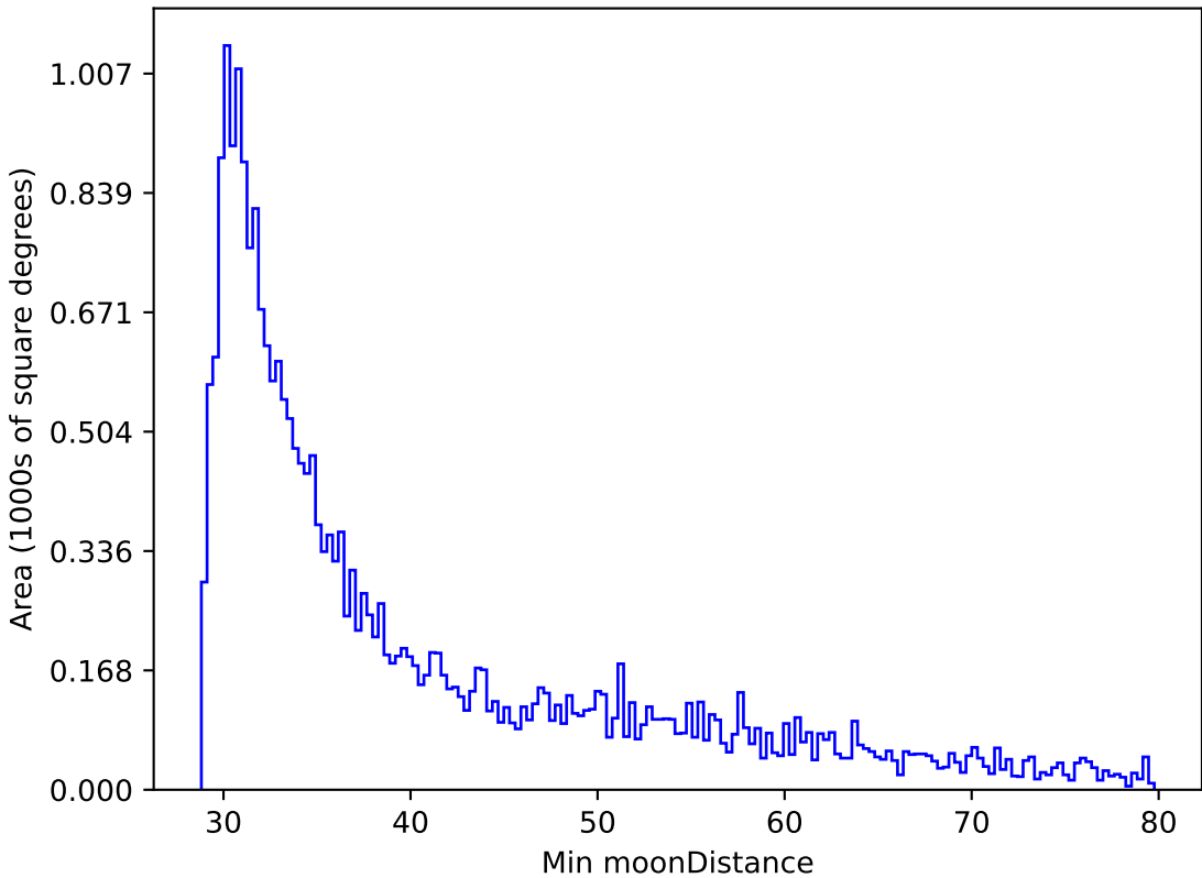
too_elab_r16_d2_giz_v3.4_10yrs All sky r band: Min moonDistance
