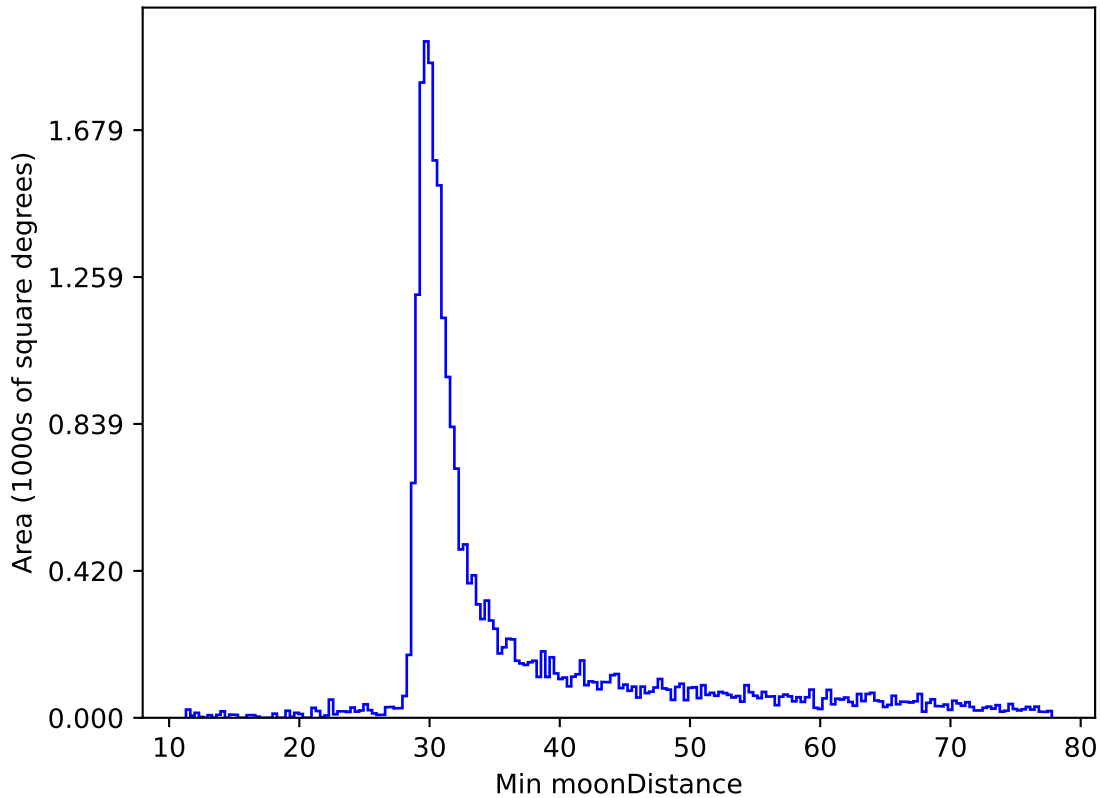
too_elab_r16_d2_giz_v3.4_10yrs All sky i band: Min moonDistance
