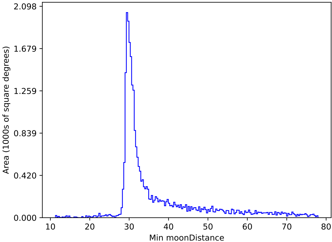
too_elab_r16_d2_giz_v3.4_10yrs All sky i band: Min moonDistance
