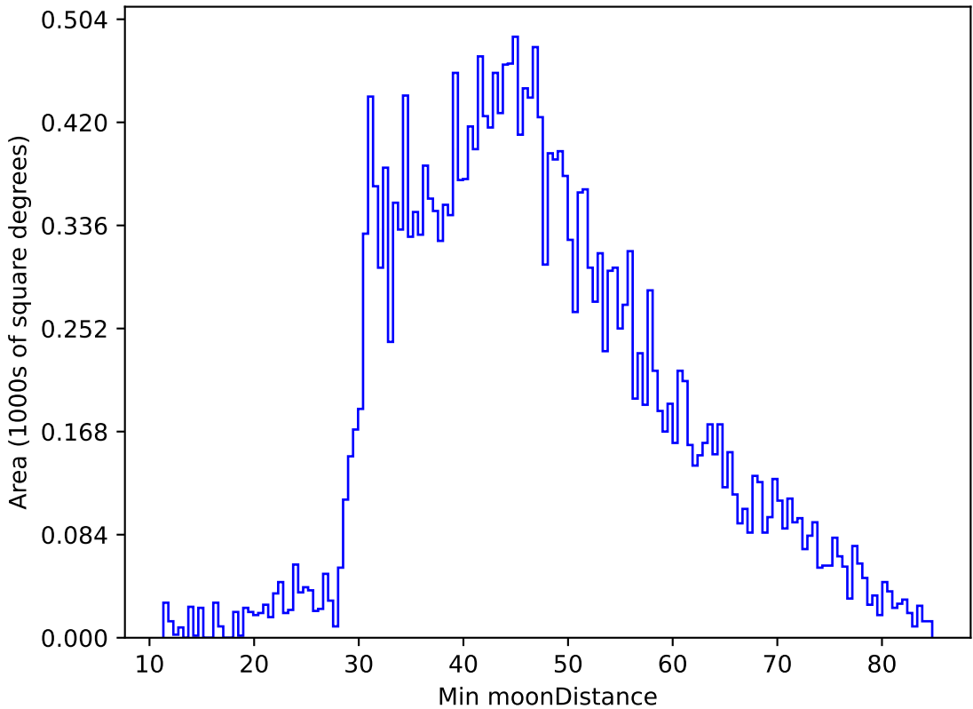
too_elab_r16_d2_giz_v3.4_10yrs All sky g band: Min moonDistance
