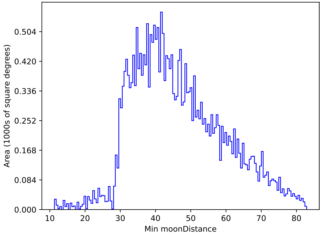
too_elab_r16_d2_giz_v3.4_10yrs All sky g band: Min moonDistance
