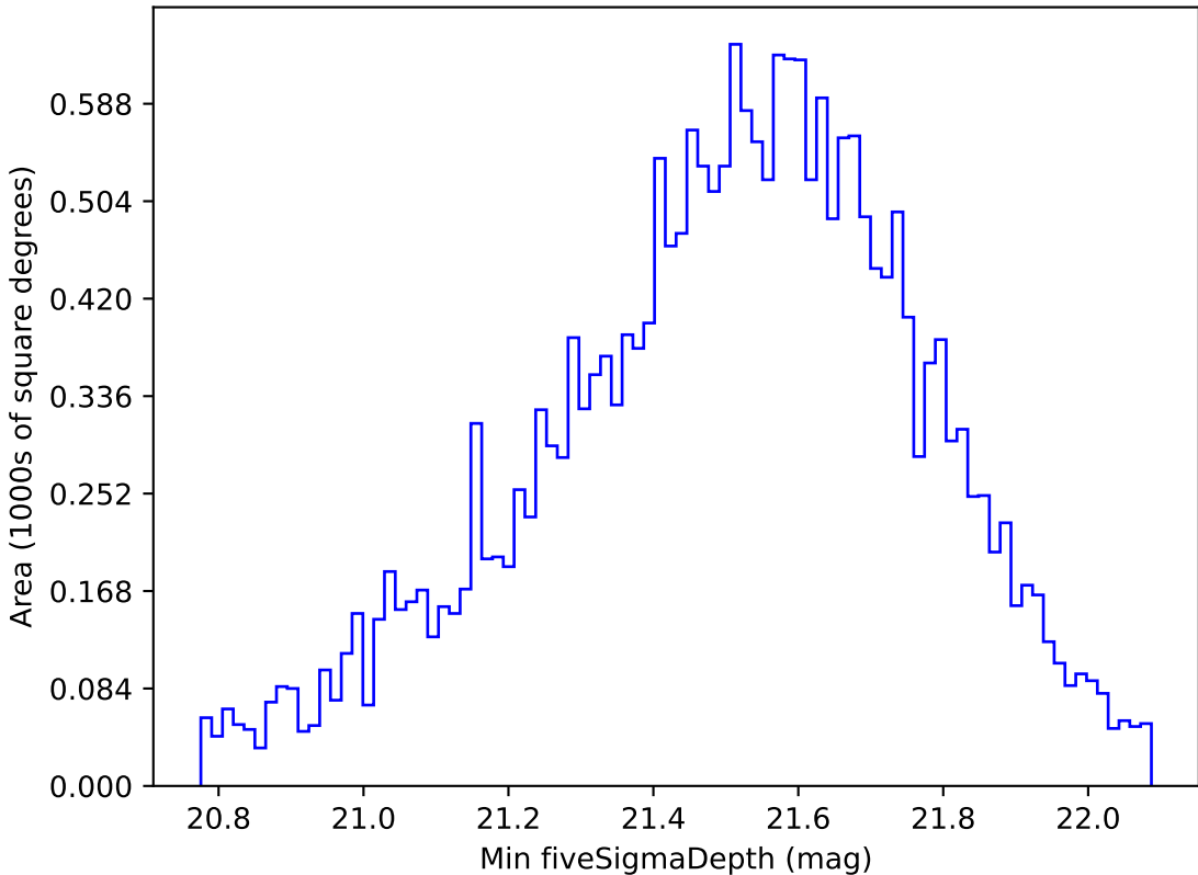
too_elab_r16_d2_giz_v3.4_10yrs Yr 1 y band: Min fiveSigmaDepth
