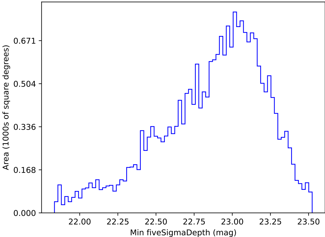
too_elab_r16_d2_giz_v3.4_10yrs Yr 1 u band: Min fiveSigmaDepth
