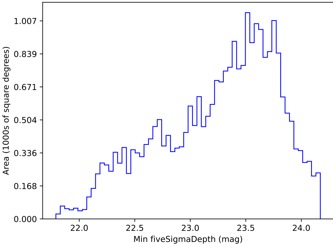
too_elab_r16_d2_giz_v3.4_10yrs Yr 1 r band: Min fiveSigmaDepth
