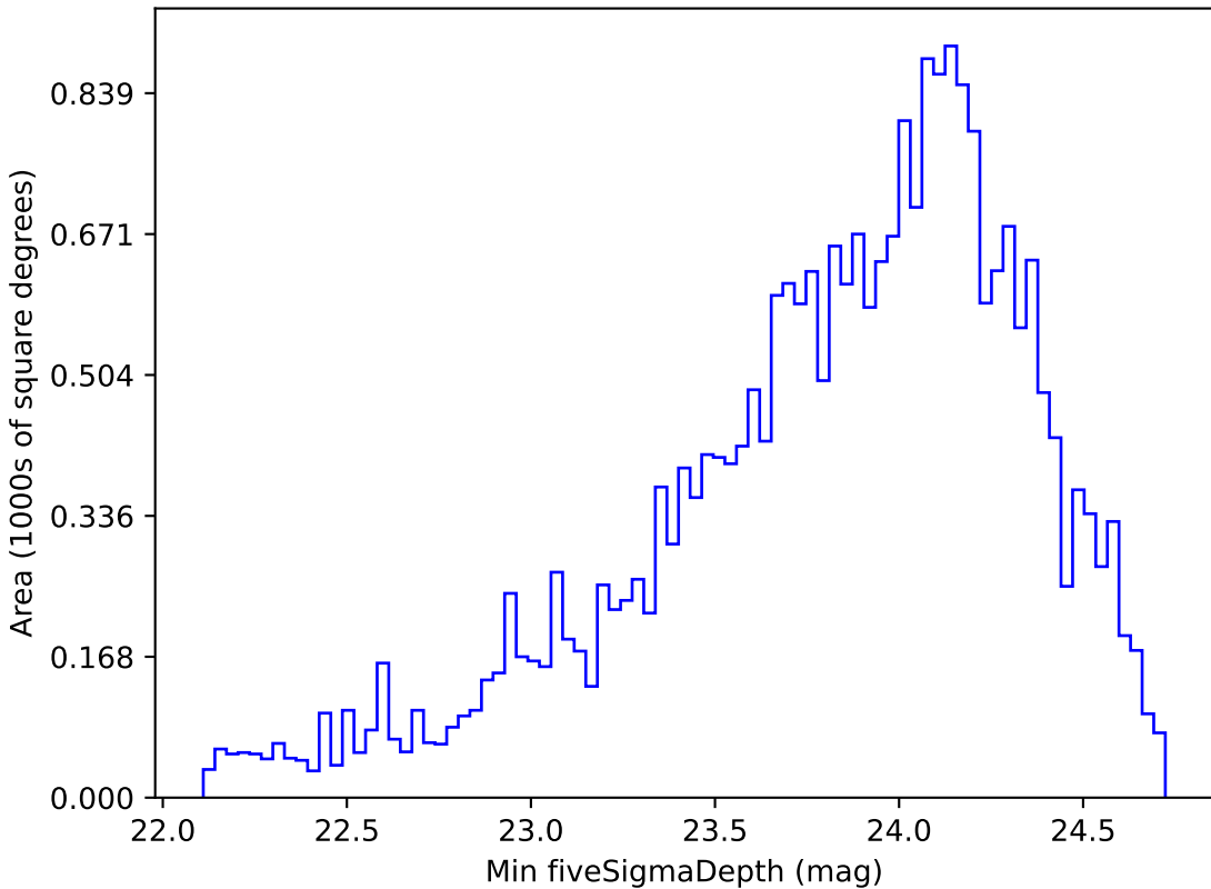
too_elab_r16_d2_giz_v3.4_10yrs Yr 1 g band: Min fiveSigmaDepth
