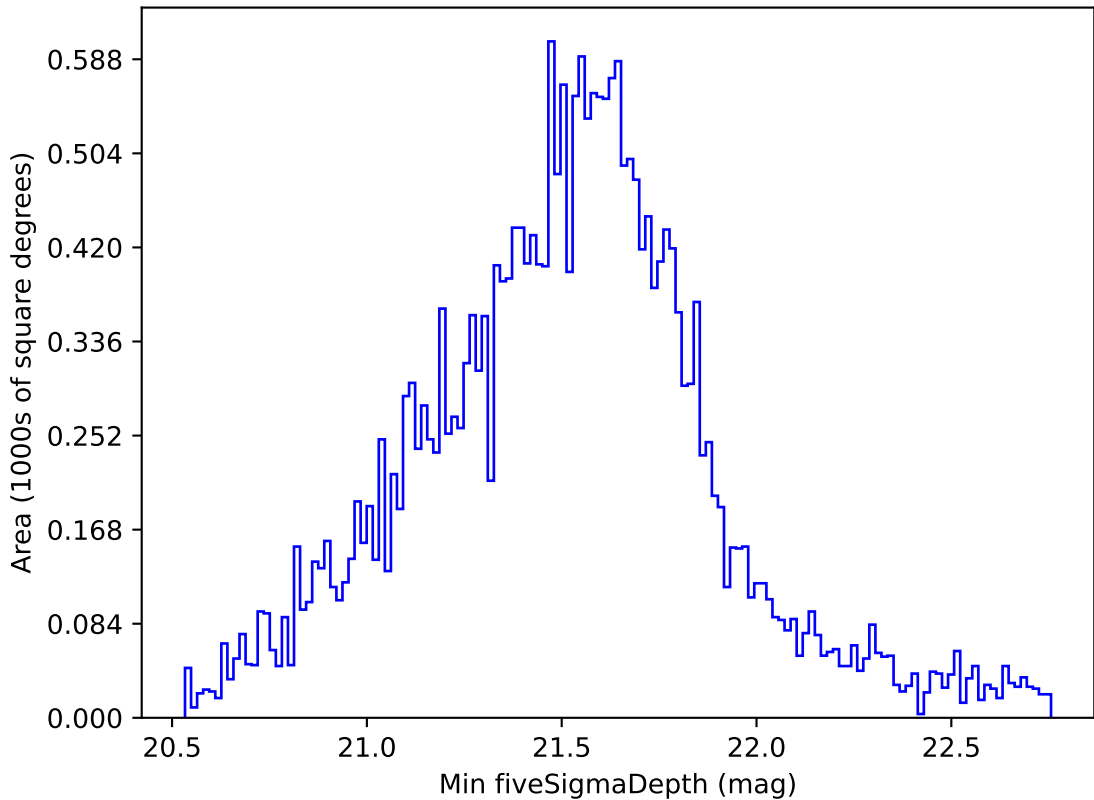
too_elab_r16_d2_giz_v3.4_10yrs Yr 1 all bands: Min fiveSigmaDepth
