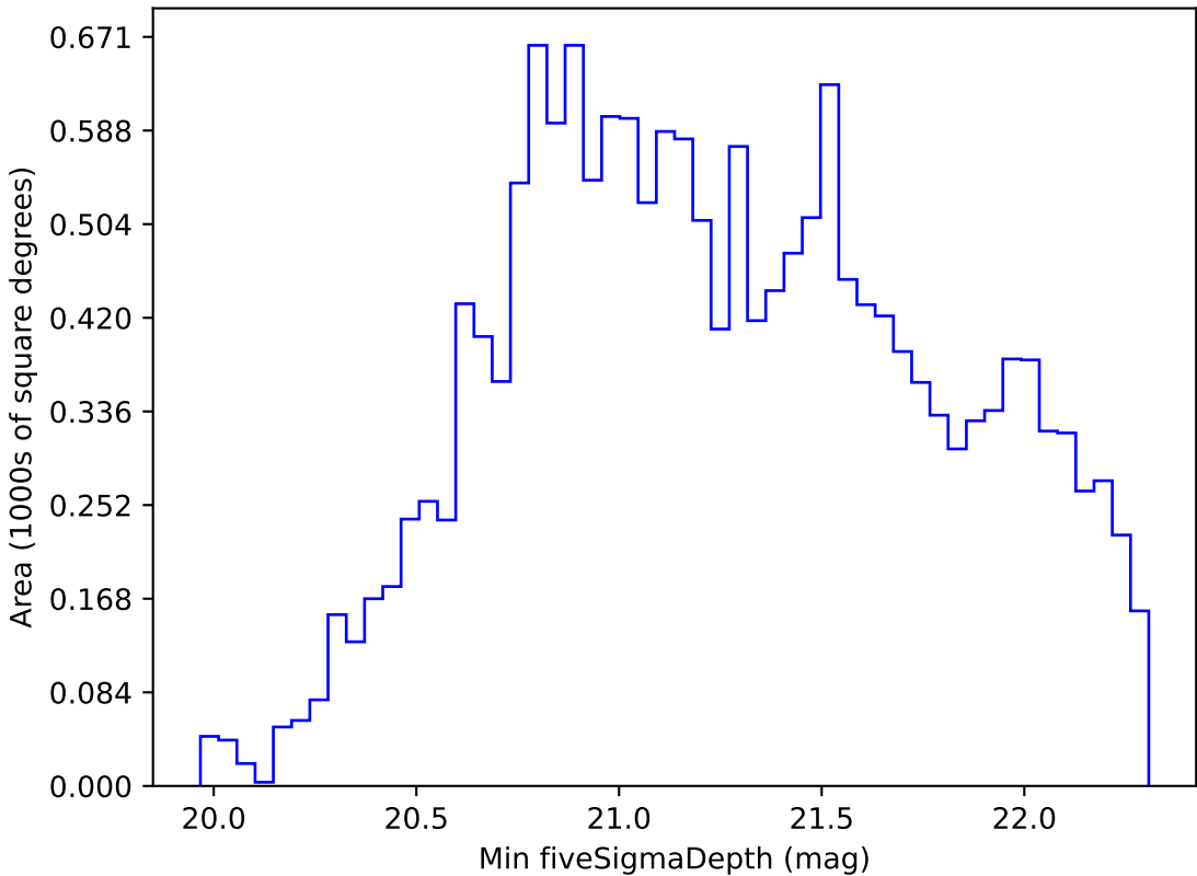
too_elab_r16_d2_giz_v3.4_10yrs WFD z band: Min fiveSigmaDepth
