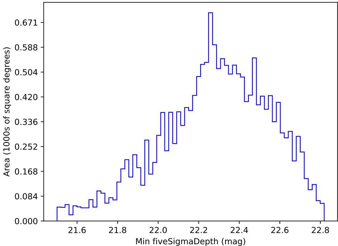
too_elab_r16_d2_giz_v3.4_10yrs WFD u band: Min fiveSigmaDepth
