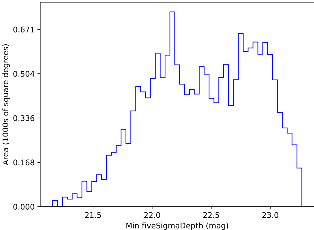
too_elab_r16_d2_giz_v3.4_10yrs WFD r band: Min fiveSigmaDepth
