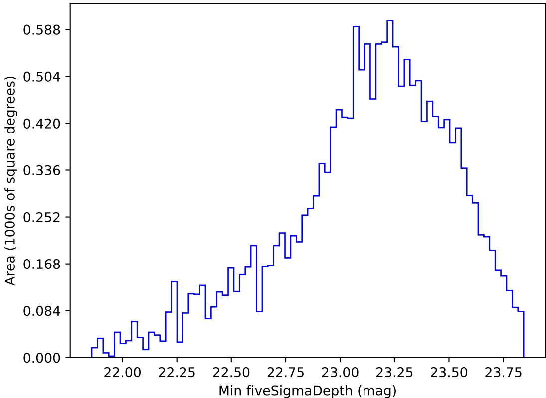
too_elab_r16_d2_giz_v3.4_10yrs WFD g band: Min fiveSigmaDepth
