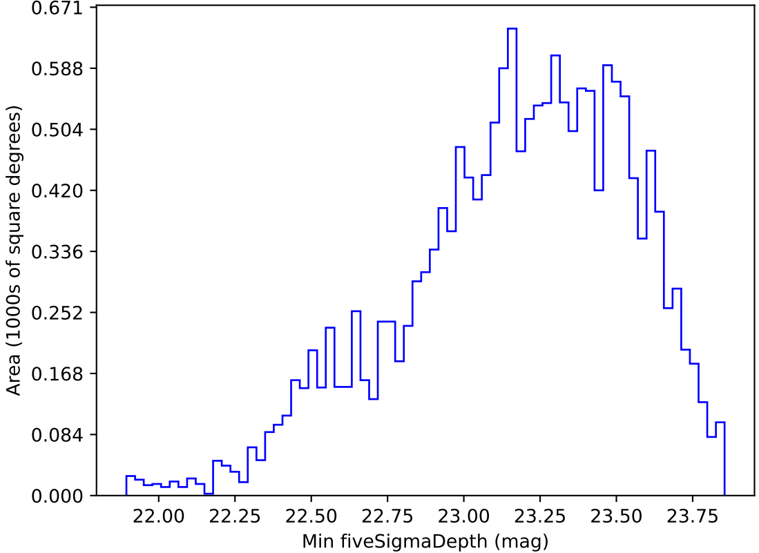
too_elab_r16_d2_giz_v3.4_10yrs WFD g band: Min fiveSigmaDepth
