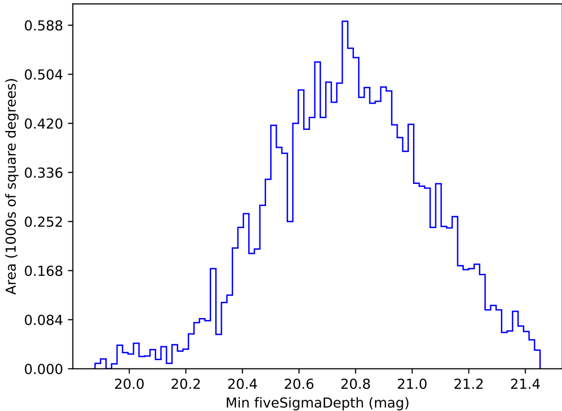
too_elab_r16_d2_giz_v3.4_10yrs WFD all bands: Min fiveSigmaDepth
