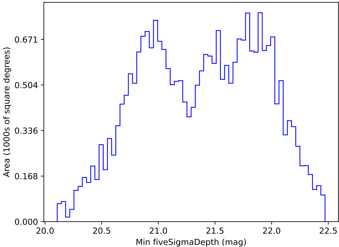
too_elab_r16_d2_giz_v3.4_10yrs All sky z band: Min fiveSigmaDepth
