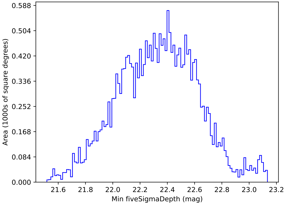
too_elab_r16_d2_giz_v3.4_10yrs All sky u band: Min fiveSigmaDepth
