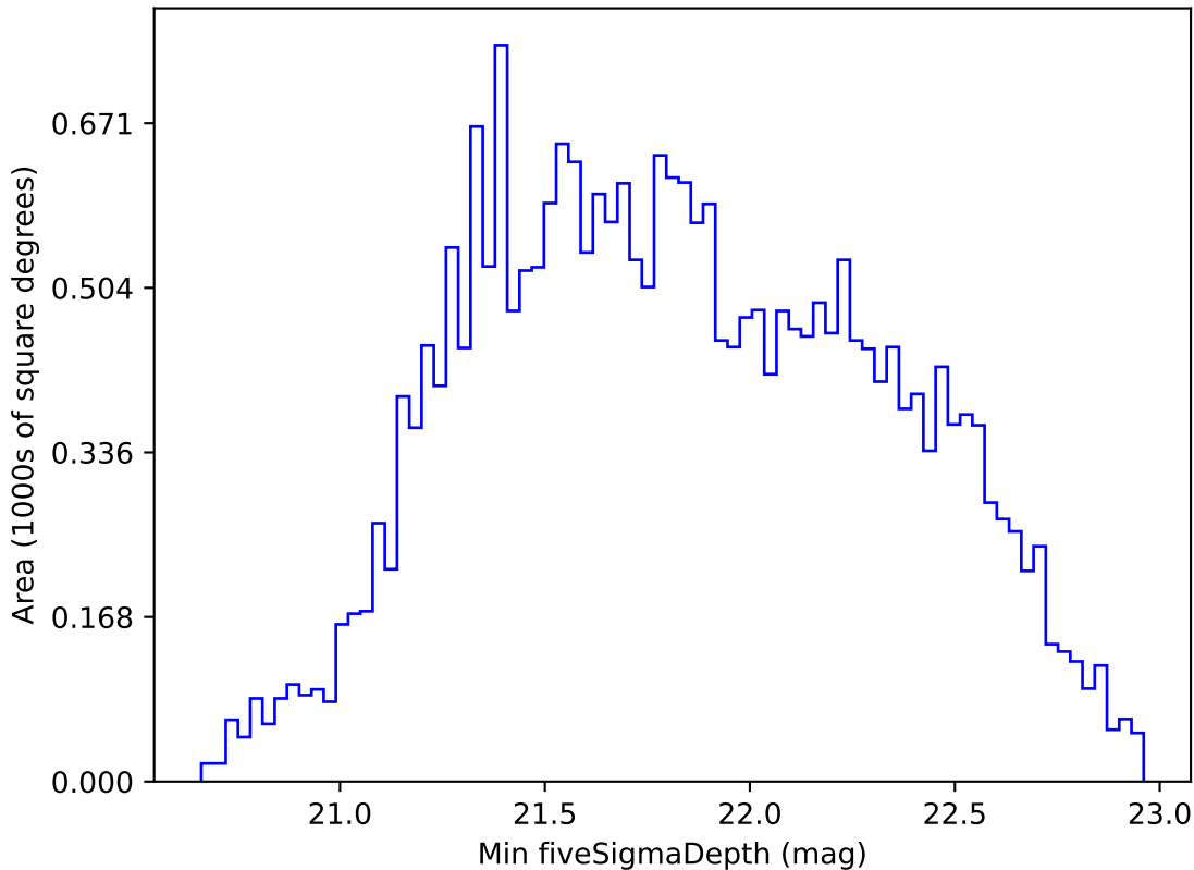
too_elab_r16_d2_giz_v3.4_10yrs All sky i band: Min fiveSigmaDepth
