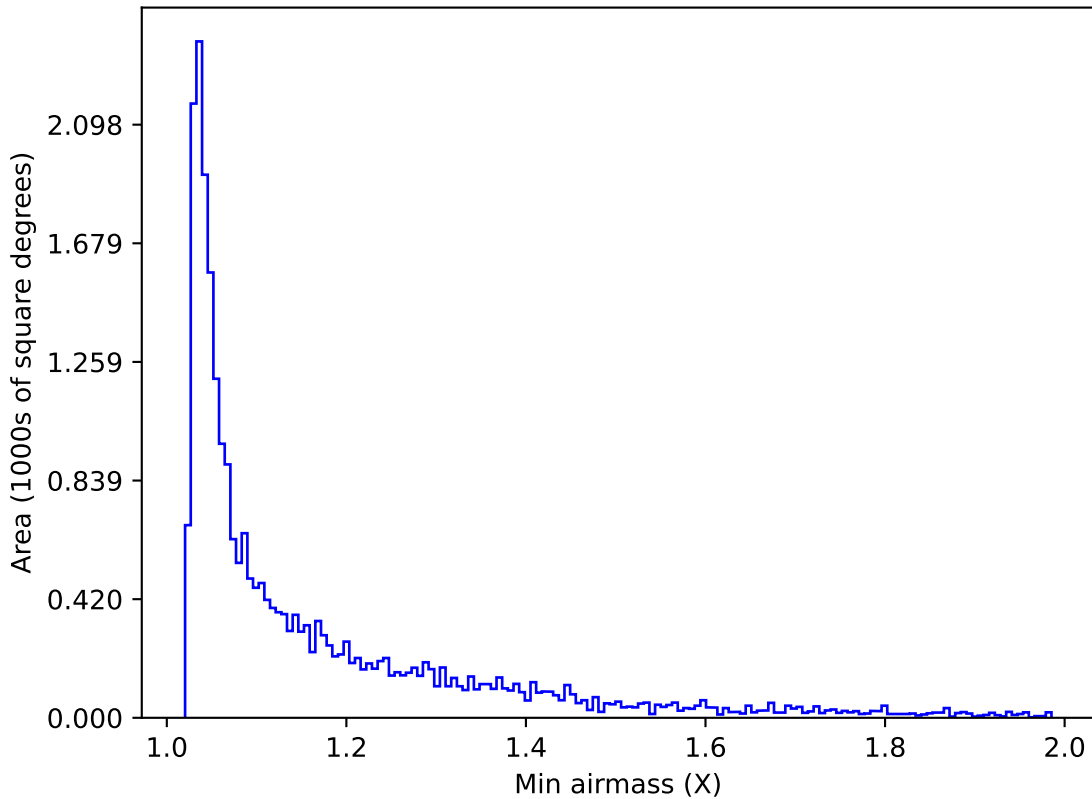
too_elab_r16_d2_giz_v3.4_10yrs Yr 1 z band: Min airmass
