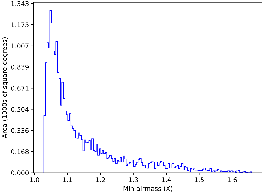
too_elab_r16_d2_giz_v3.4_10yrs Yr 1 u band: Min airmass
