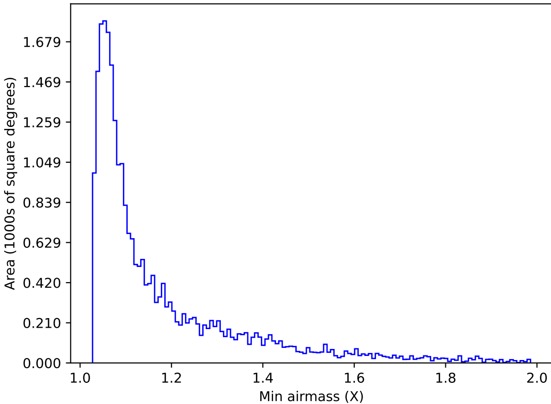
too_elab_r16_d2_giz_v3.4_10yrs Yr 1 g band: Min airmass
