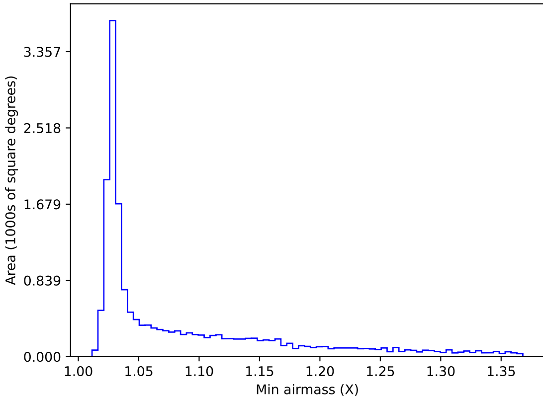
too_elab_r16_d2_giz_v3.4_10yrs WFD z band: Min airmass
