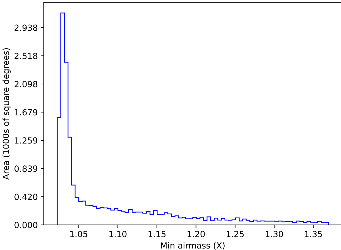
too_elab_r16_d2_giz_v3.4_10yrs WFD y band: Min airmass
