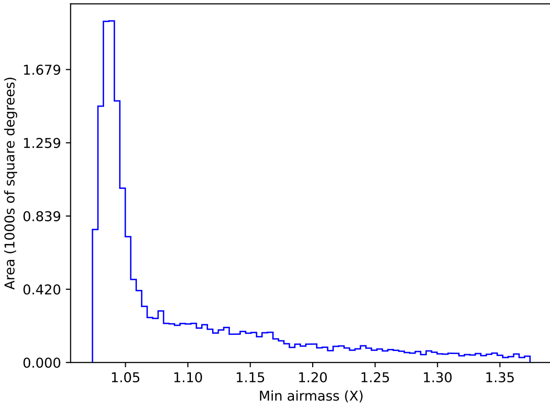
too_elab_r16_d2_giz_v3.4_10yrs WFD u band: Min airmass
