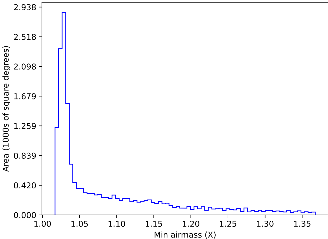
too_elab_r16_d2_giz_v3.4_10yrs WFD r band: Min airmass
